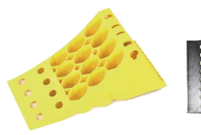
Model(型号):WC-11 Size: 475 × 200 × 235mm Weight: 1.6kg
