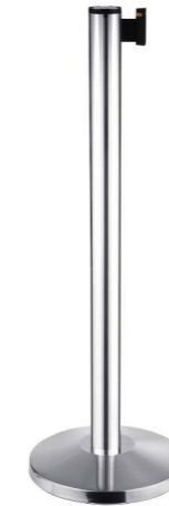
亮光铝槽款 Mirror Aluminum Barrier Size(尺寸):350x70x1020mm Weight(重量):10.5kg
