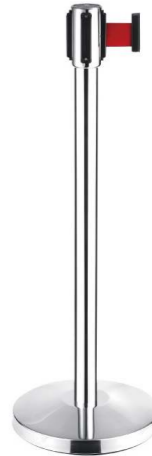
51管配铝槽拉带头款 Dia51 Aluminum Head Barrier Size(尺寸):350x51x1020mm Weight(重量):10kg
