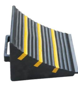
Model(型号):WC-06 Size: 320 × 290 × 260mm Weight: 12kg
